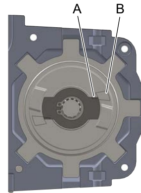
Figure 12. Brake Alignment
