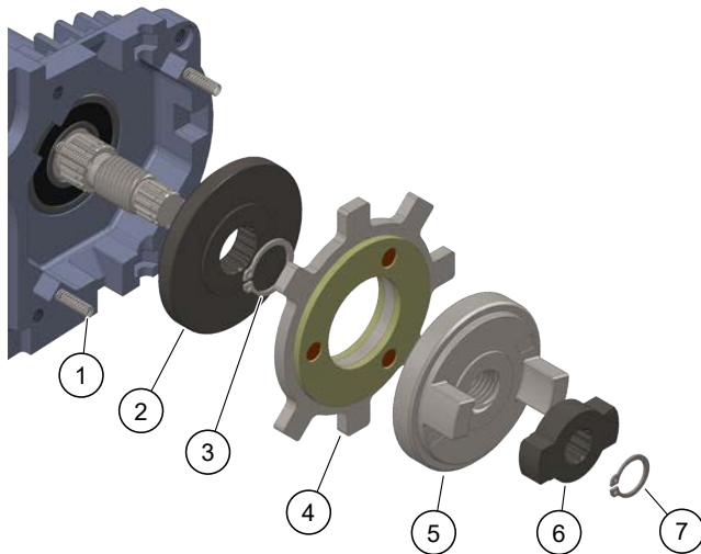
Figure 11. Brake Assembly
