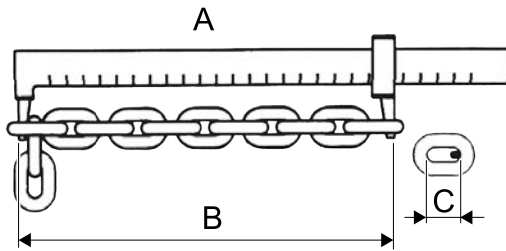
Figure 9. Gaging Load Chain Wear
