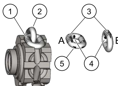
Figure 7. Chain Wear Areas
