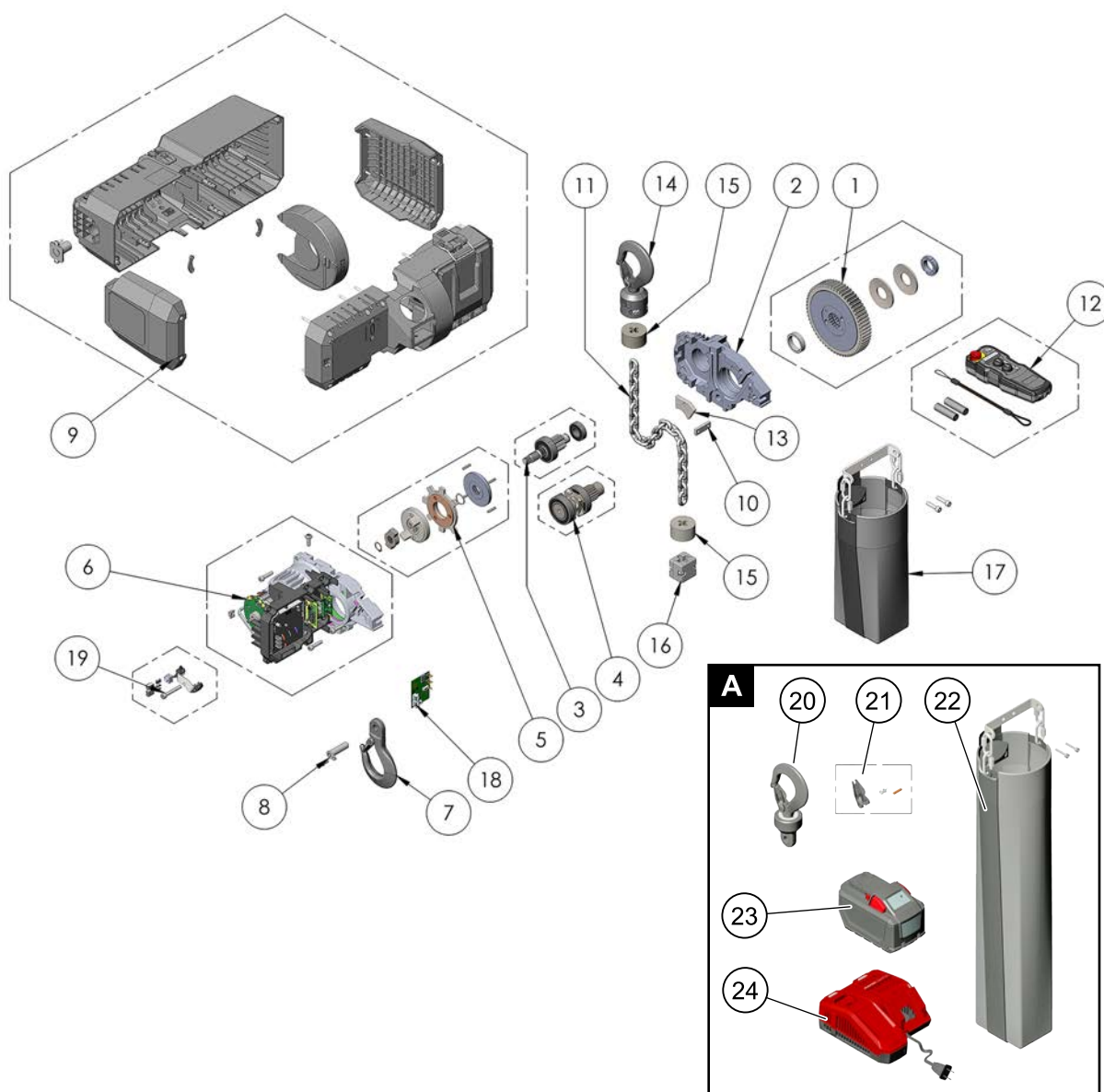
Figure 14. Hoist Parts
